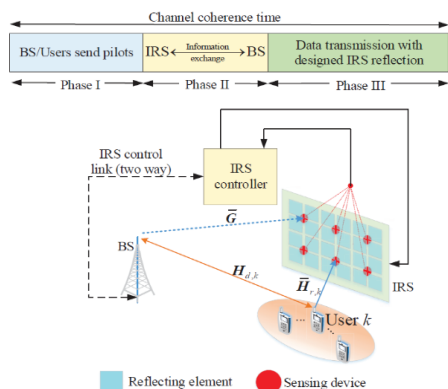
(a) Semi-passive IRS.
