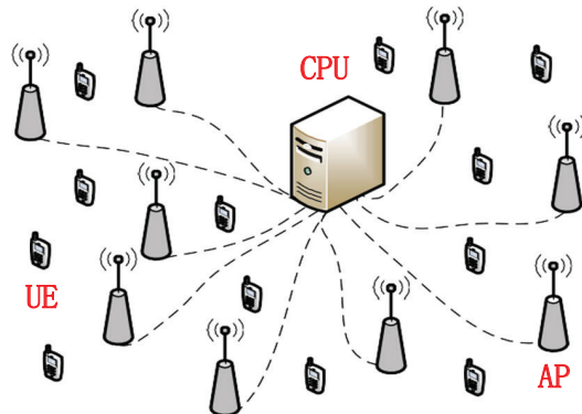
(a) conventional cell-free massive MIMO system.
