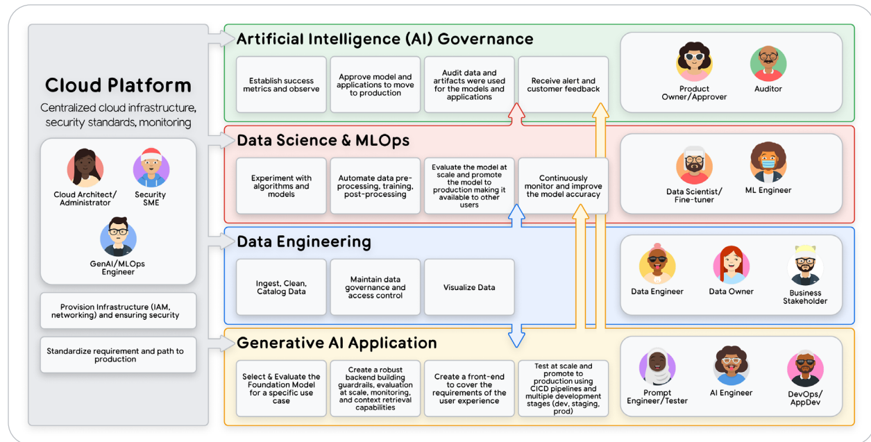
Figure 2: How multiple teams collaborate to operationalize both models and GenAI applications
