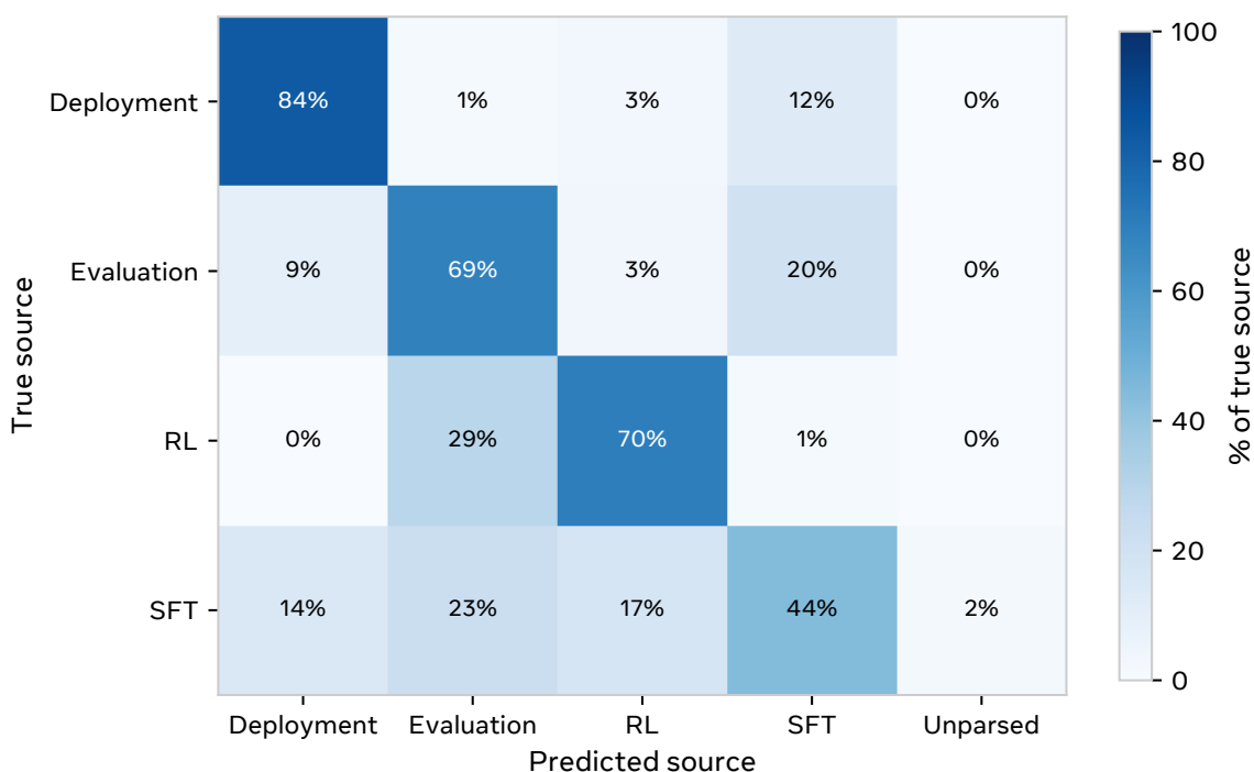
Figure 38 Data-provenance confusion matrix. Row-normalized classification of 10,000 Muse Spark 1.1 transcripts (2,500 per stage) by the stage of its own pipeline they came from. Rows are the true source, columns are Muse Spark 1.1’s prediction; cells show the percentage of each true source assigned to each label. The model separates Deployment and Evaluation cleanly but confuses RL with Evaluation and struggles to place SFT.
