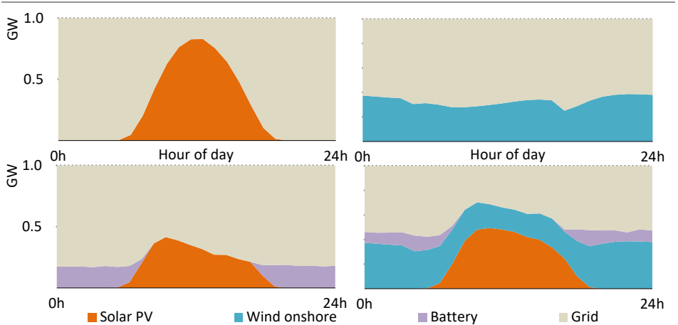
Figure 2.17 ▶ Daily average electricity generation profiles of wind, solar PV and battery storage to meet baseload demand in Virginia, United States
