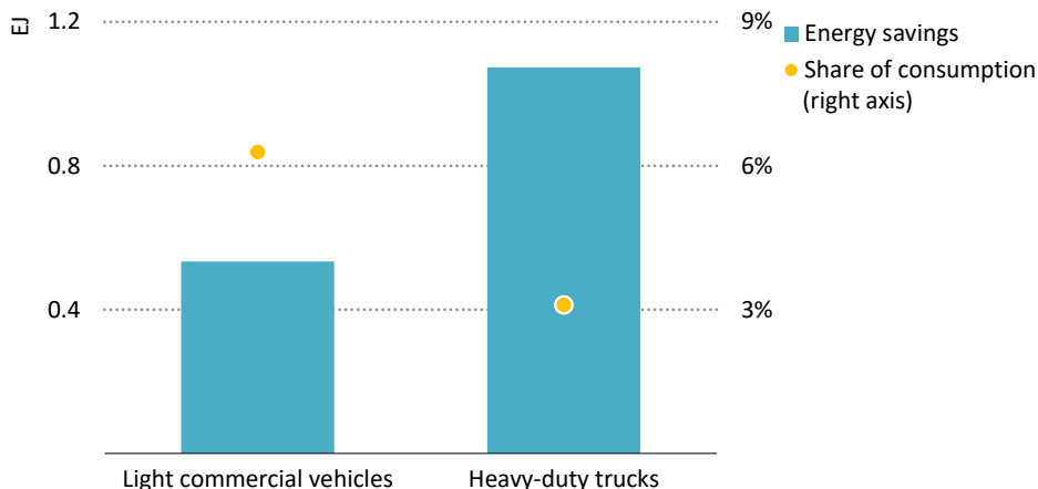
Figure 3.13 ▶ Energy savings in road freight in the Widespread Adoption Case, 2035
