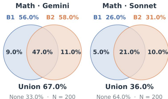
Figure 2(b), math panels. 200 tasks per model. Circle areas are schematic.
