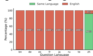
(b) Reasoning language: the language the model GLM 4.7 Z.ai et al. (2025) reasons in.
