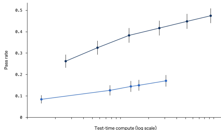
Performance of GPT-6 Astra and our Internal Model on a curated set of open math problems
