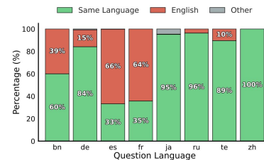
(d) Reasoning language: the language the model MIMO-V2-Flash reasons in.
