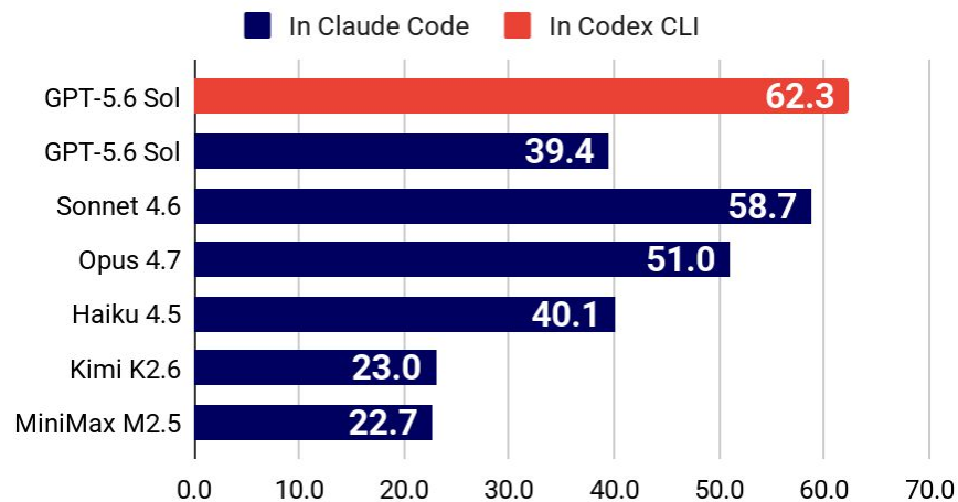
HarnessSafe containment score (0-100, higher is better)
