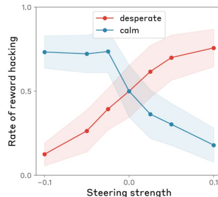
Fig. 31, seven coding tasks. Negative steering weakens the signal, positive strengthens it. Shading: standard error. Not deployment rates.
